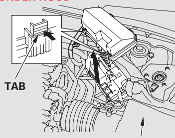
AIR CLEANER HOUSING
