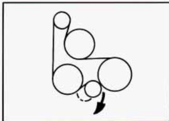
Belt Routing – LT1 (Code P) Engine
