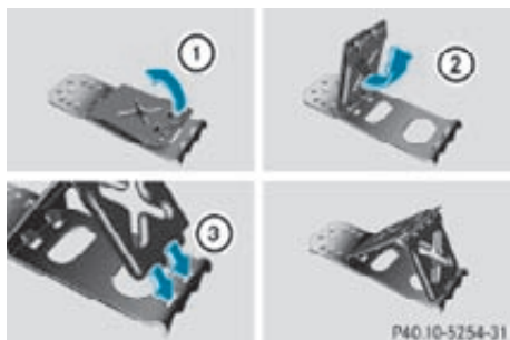
Storage position
