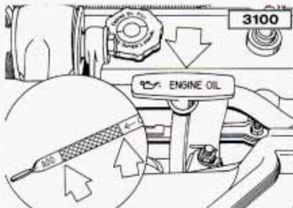
3100 V6: Checking Engine Oil
