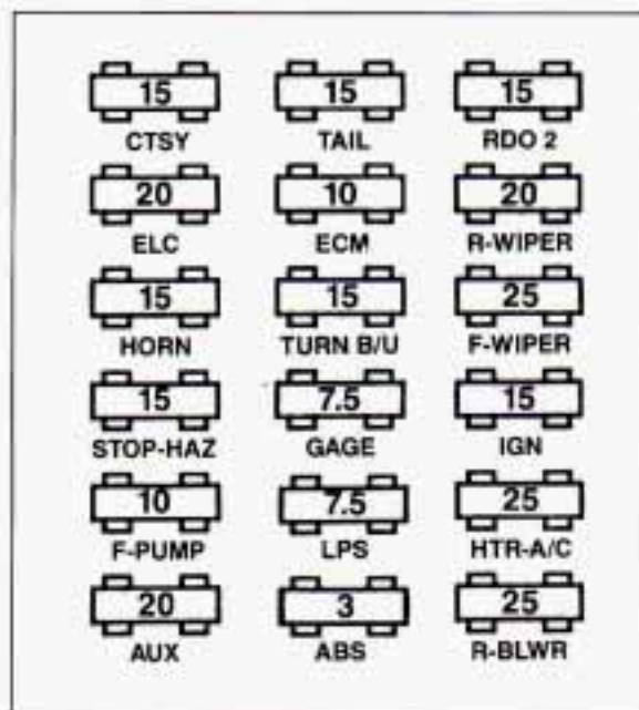
Fuse Panel (3100 V6 ENGINE)
