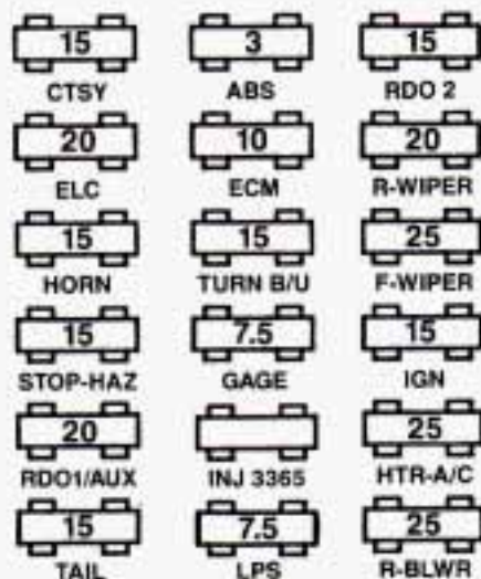
Fuse Panel (3800 V6 ENGINE)
