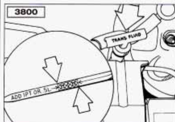
3800 V6: Checking Automatic Transaxle Fluid
