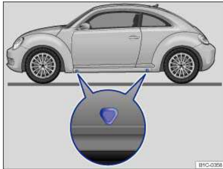
Fig. 161 Lift points for the jack.
