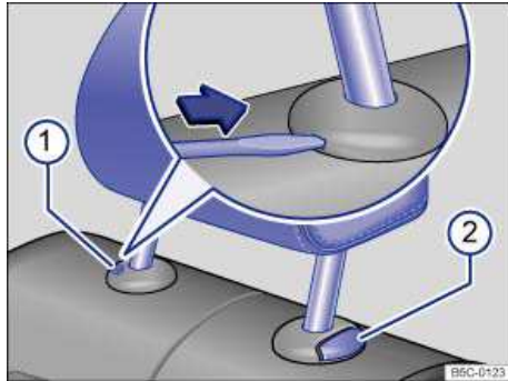
Fig. 39 Removing the rear head restraints.
