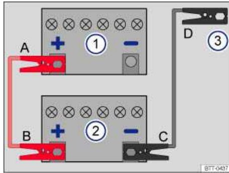
Fig. 182 Diagram for attaching the jumper cables: Dead battery 1 and booster battery 2.
