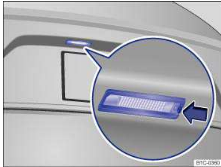
Fig. 180 In the rear bumper: License plate light.
