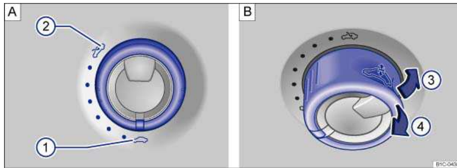
Fig. 32 In the headliner: Rotary switch for the power sunroof. A: Turn the rotary switch to slide the sunroof open or closed. B: Press or pull the switch to tilt open or to close.
