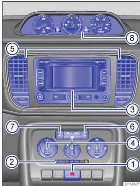
Fig. 6 Overview of the upper center console.
