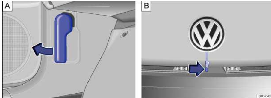
Fig. 137 A: In the footwell on the driver side: Inside engine hood release lever. B: Above the radiator grille: Outside engine hood release.
