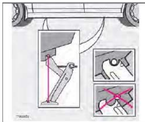
Attaching the jack
