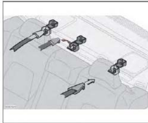
Top tether anchorage points
