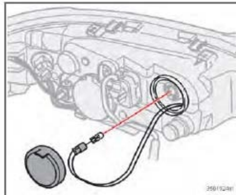
(Active Bi-Xenon® headlights)
