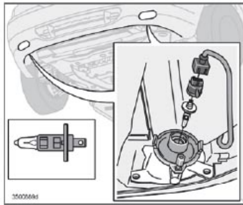
Front fog light
